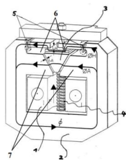
Fig. 7 OCT device.
