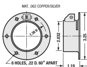
FM2D Flange Mount
